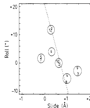
FIGURE 7: Roll-slide diagram for the restrained energy minimized average structure (RD)m. The dashed line from roll, slide = -10^\circ , 1 Å to +20^\circ , 0.2 Å represents the break between A- and B-type DNA geometries, which lie to the right and left, respectively, of the line (Calladine & Drew, 1984).
